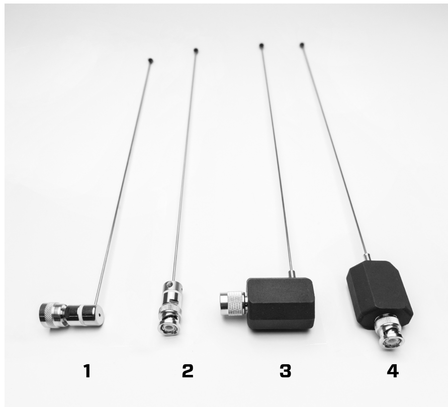
A. 13" SHORT WHIP ANTENNAS
